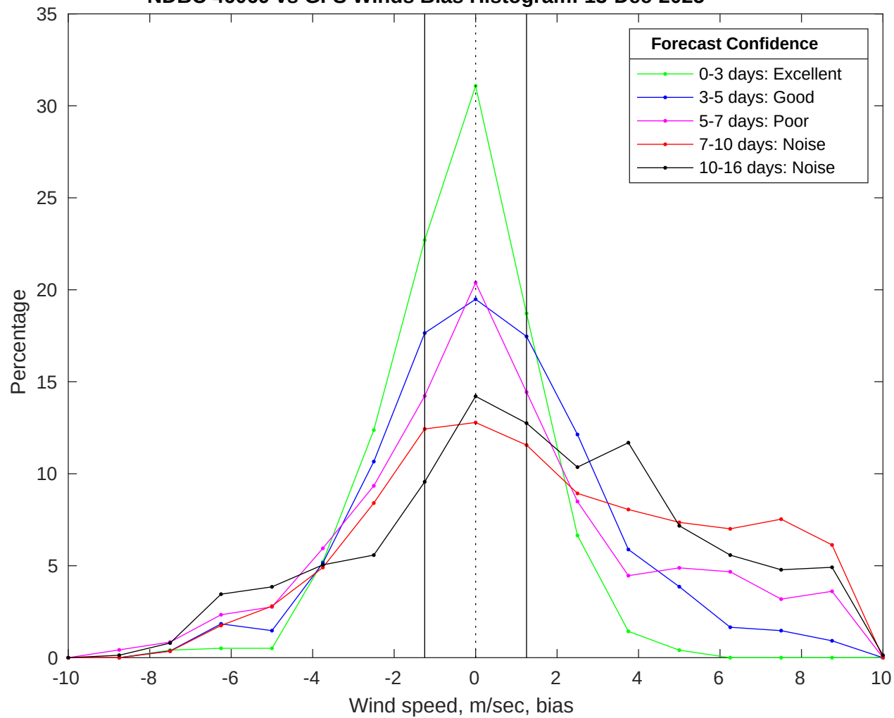
NDBC 46069 vs GFS Winds Bias Histogram: 13-Dec-2025
