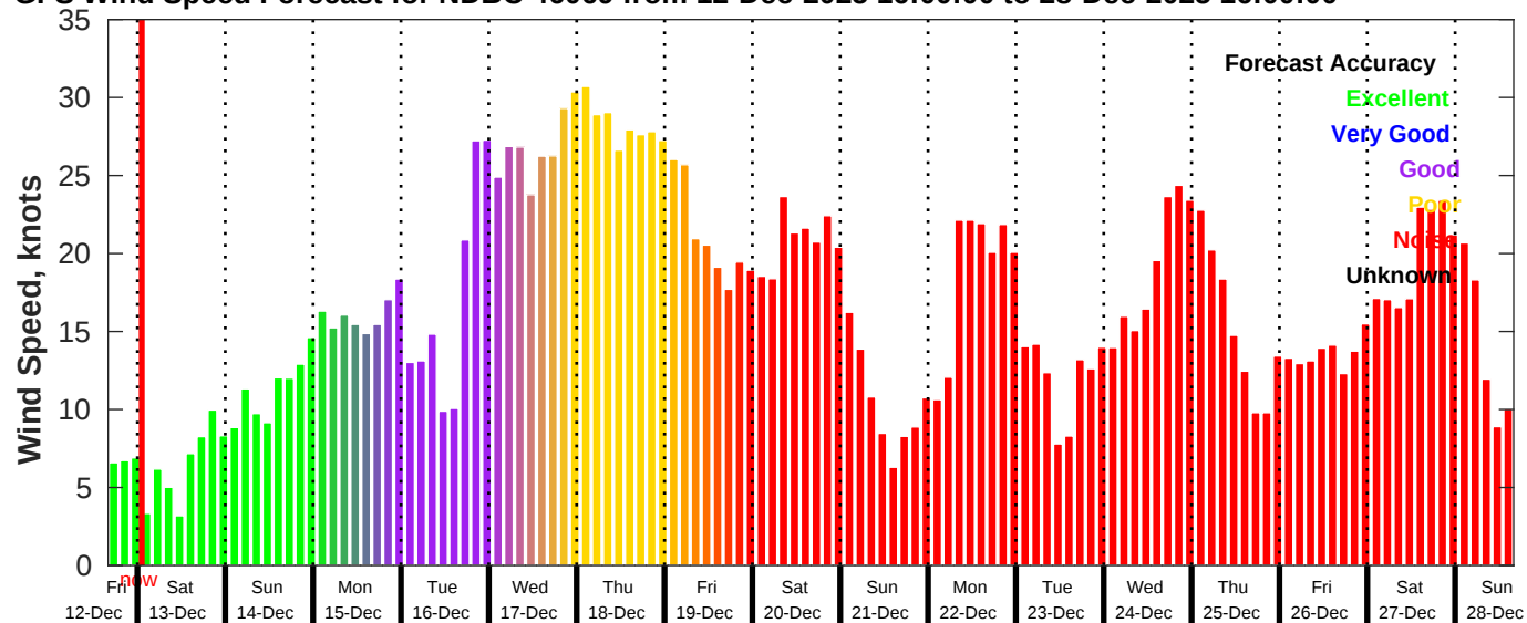
GFS Wind Speed Forecast for NDBC 46069 from 12-Dec-2025 16:00:00 to 28-Dec-2025 16:00:00
