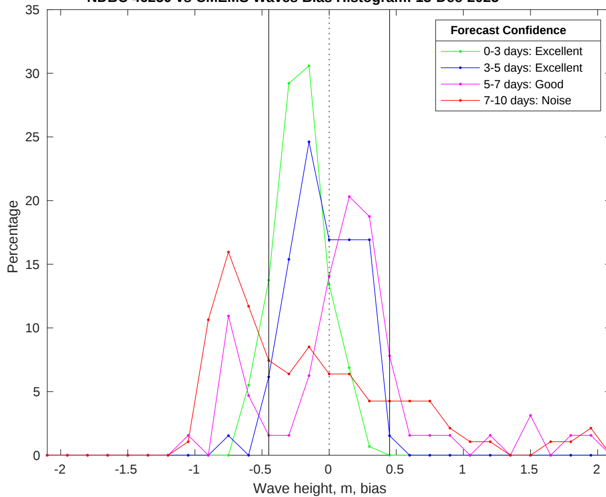
NDBC 46259 vs CMEMS Waves Bias Histogram: 13-Dec-2025
