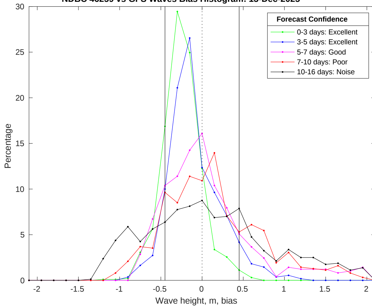
NDBC 46259 vs GFS Waves Bias Histogram: 13-Dec-2025
