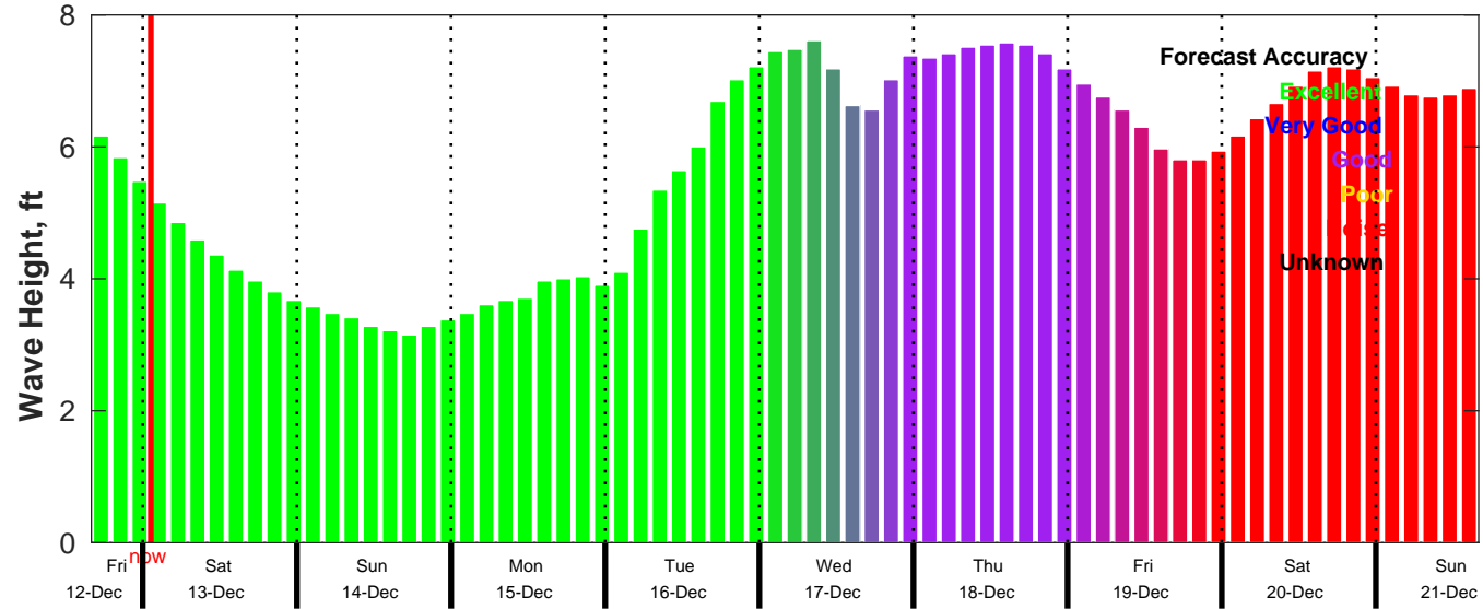
CMEMS Wave Forecast for NDBC 46259 from 12-Dec-2025 16:00:00 to 21-Dec-2025 16:00:00
