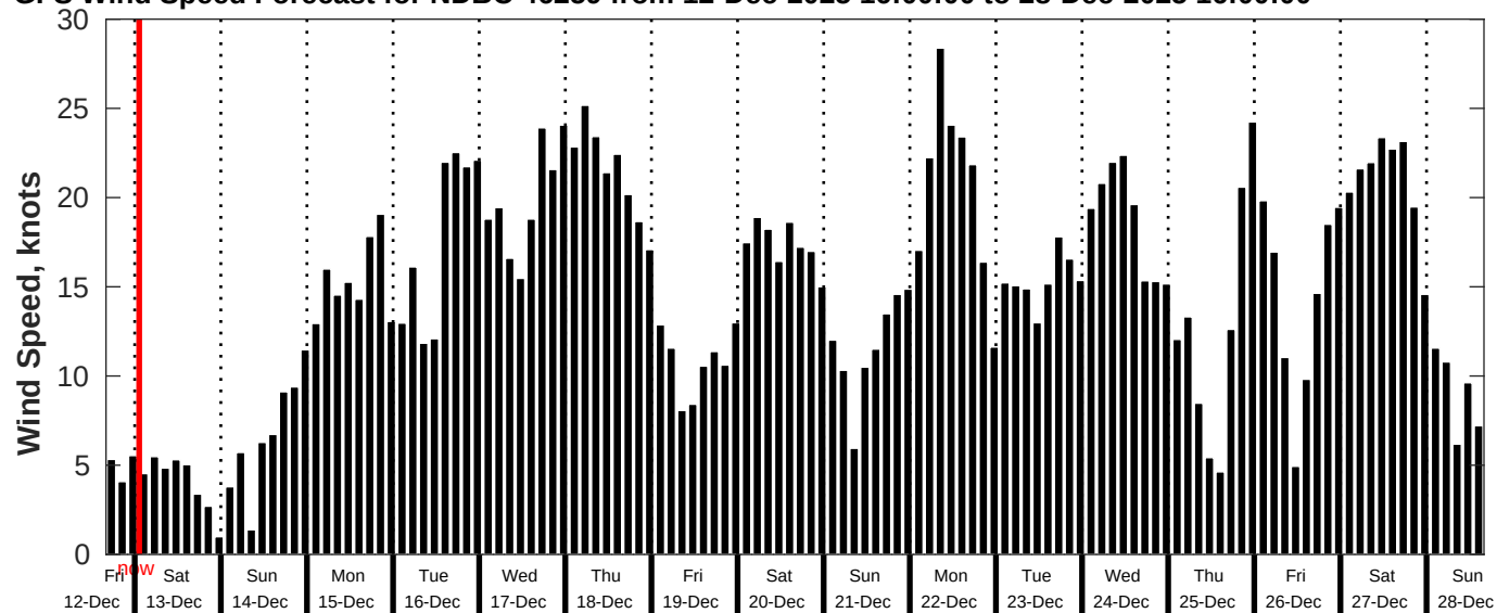
GFS Wind Speed Forecast for NDBC 46259 from 12-Dec-2025 16:00:00 to 28-Dec-2025 16:00:00
