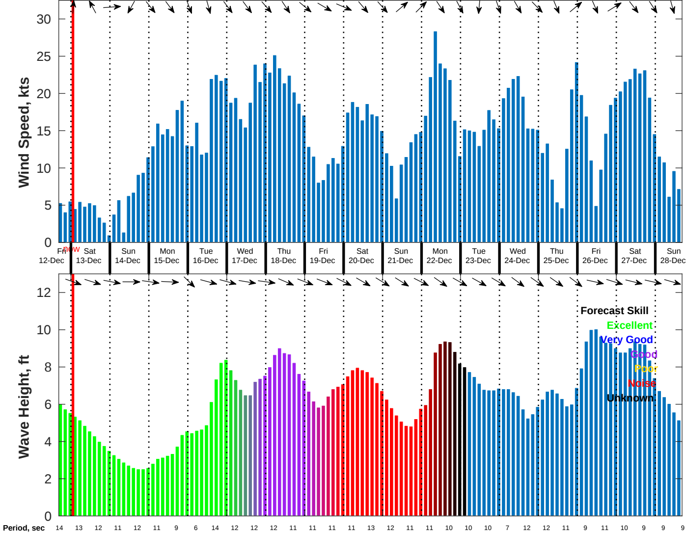
Wind & Wave Forecast for NDBC 46259 from 12-Dec-2025 16:00:00 to 28-Dec-2025 16:00:00
