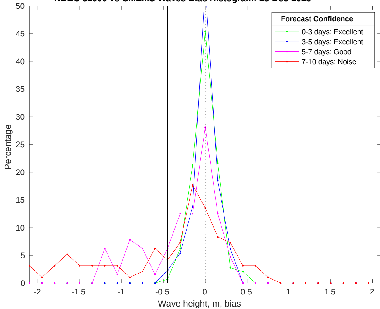
NDBC 51000 vs CMEMS Waves Bias Histogram: 13-Dec-2025
