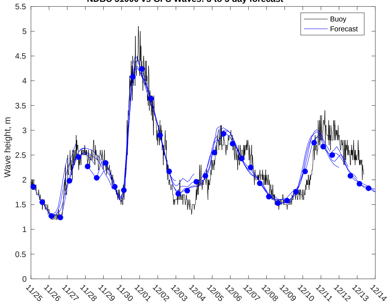
NDBC 51000 vs GFS Waves: 3 to 5 day forecast
