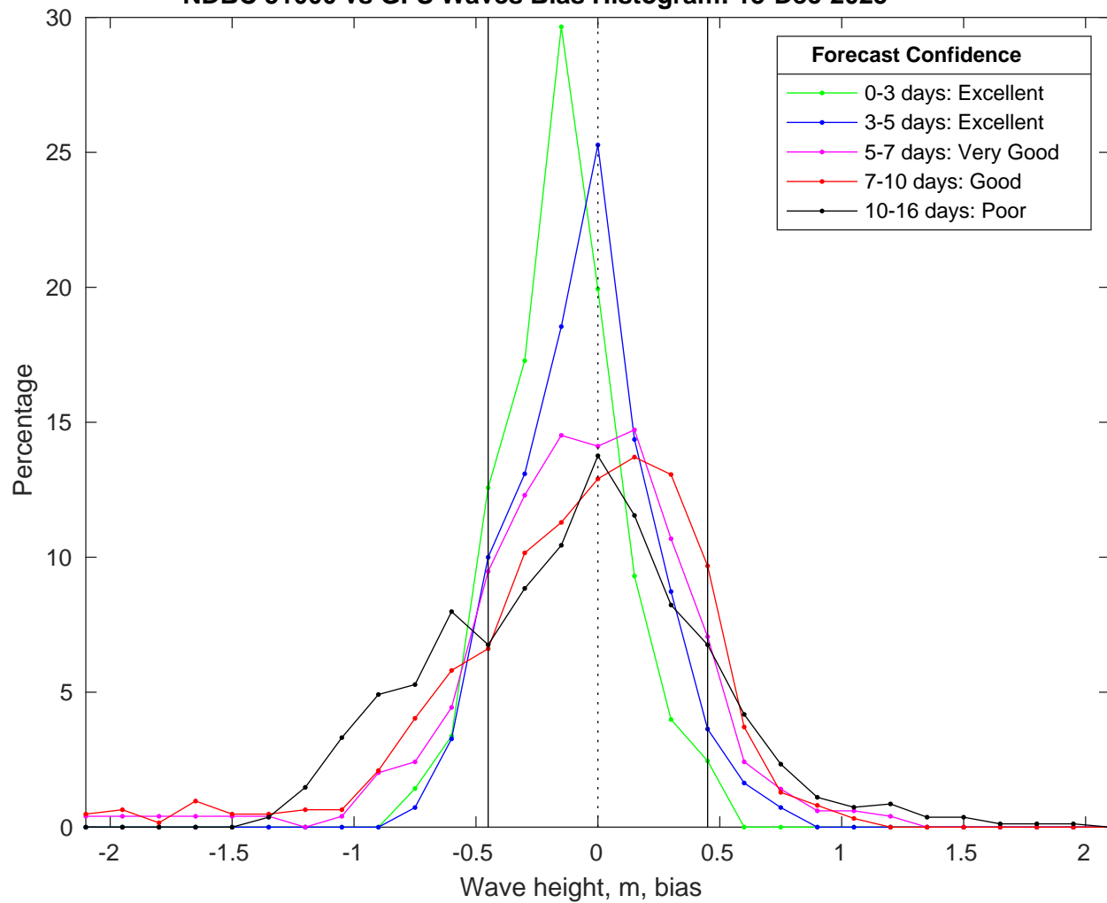
NDBC 51000 vs GFS Waves Bias Histogram: 13-Dec-2025
