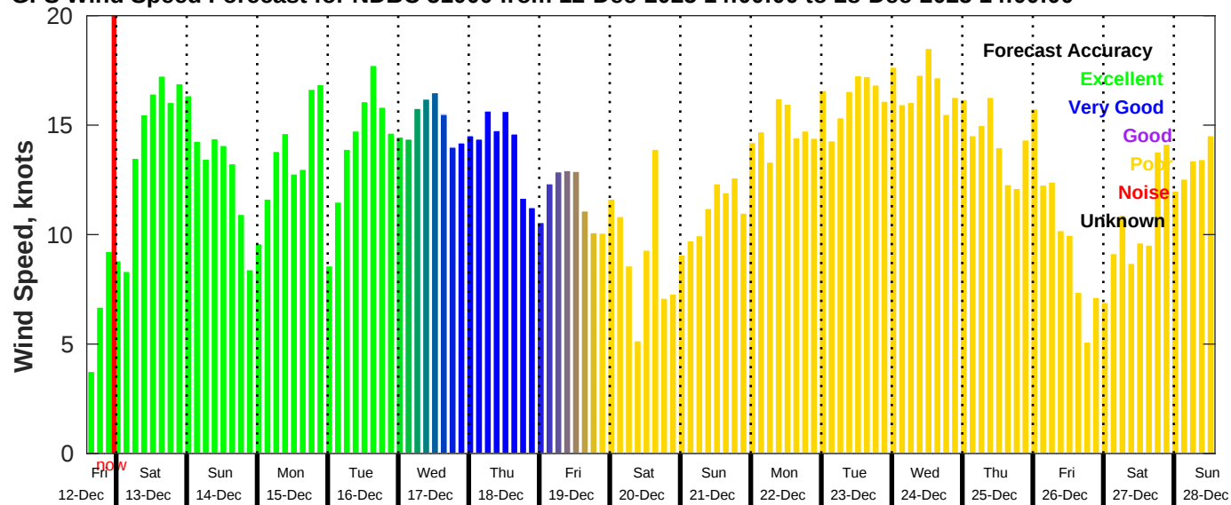
GFS Wind Speed Forecast for NDBC 51000 from 12-Dec-2025 14:00:00 to 28-Dec-2025 14:00:00
