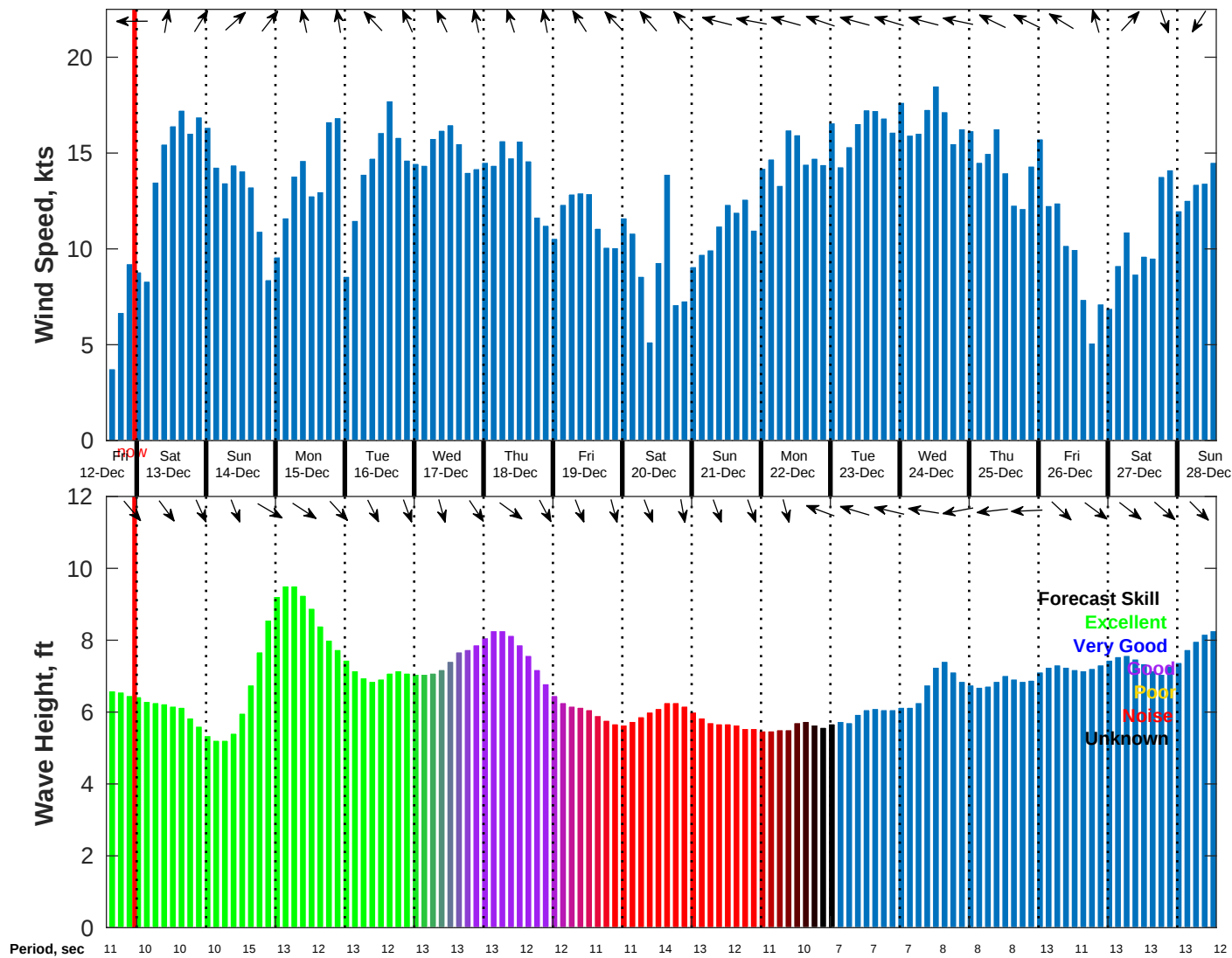
Wind & Wave Forecast for NDBC 51000 from 12-Dec-2025 14:00:00 to 28-Dec-2025 14:00:00
