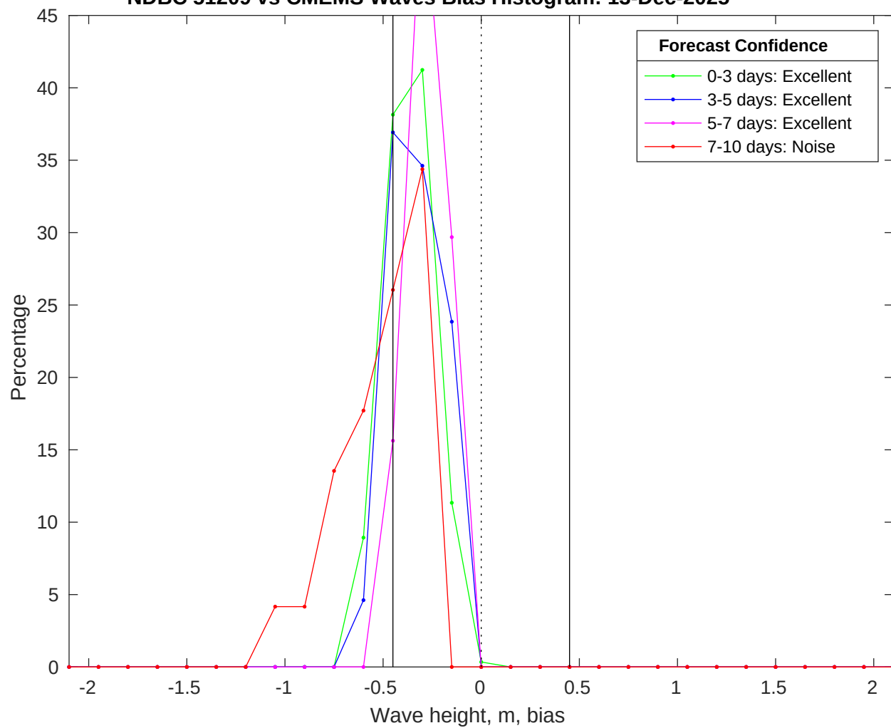
NDBC 51209 vs CMEMS Waves Bias Histogram: 13-Dec-2025
