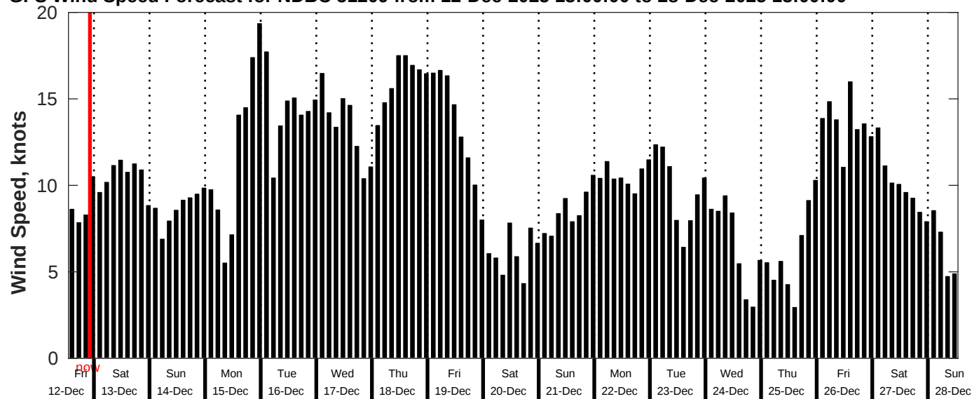
GFS Wind Speed Forecast for NDBC 51209 from 12-Dec-2025 13:00:00 to 28-Dec-2025 13:00:00
