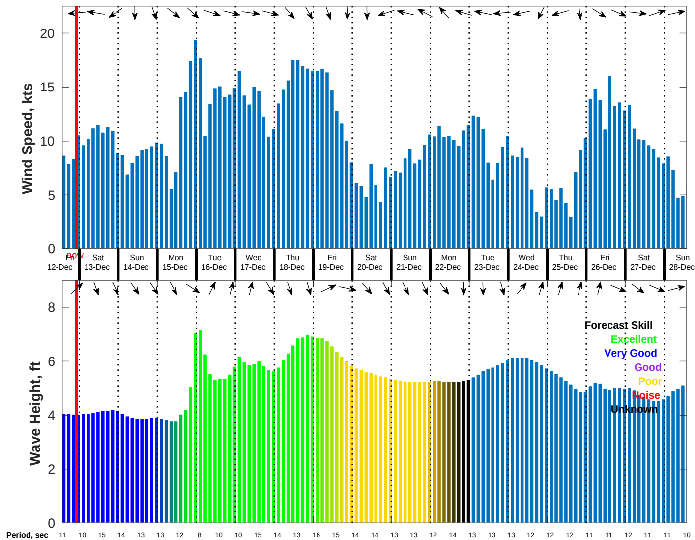
Wind & Wave Forecast for NDBC 51209 from 12-Dec-2025 13:00:00 to 28-Dec-2025 13:00:00
