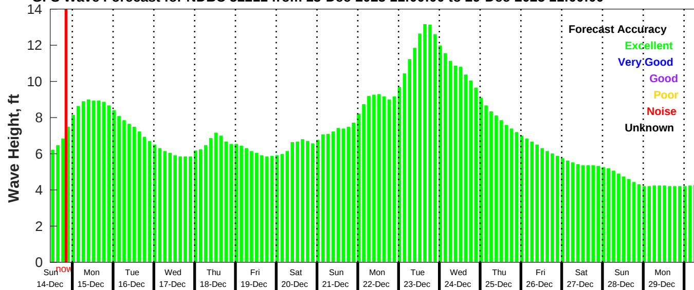
GFS Wave Forecast for NDBC 52211 from 13-Dec-2025 11:00:00 to 29-Dec-2025 11:00:00
