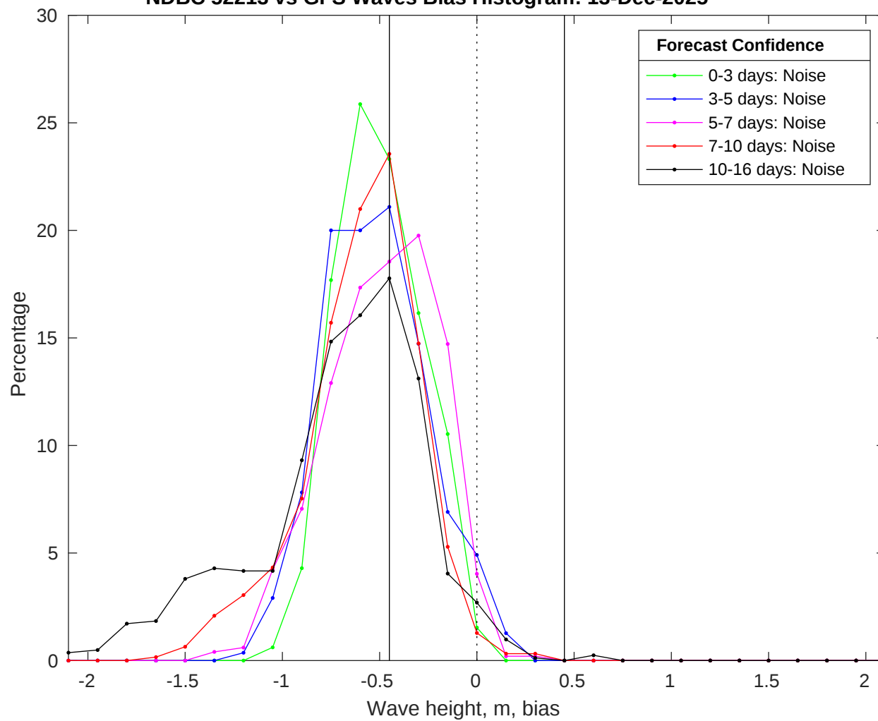
NDBC 52213 vs GFS Waves Bias Histogram: 13-Dec-2025
