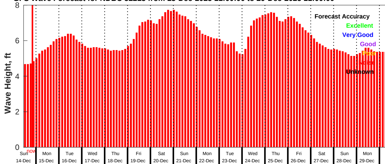
GFS Wave Forecast for NDBC 52213 from 13-Dec-2025 11:00:00 to 29-Dec-2025 11:00:00
