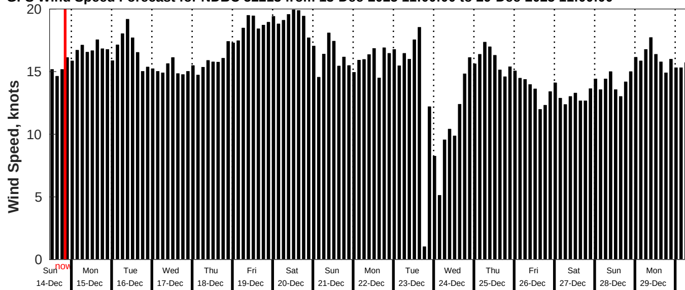
GFS Wind Speed Forecast for NDBC 52213 from 13-Dec-2025 11:00:00 to 29-Dec-2025 11:00:00
