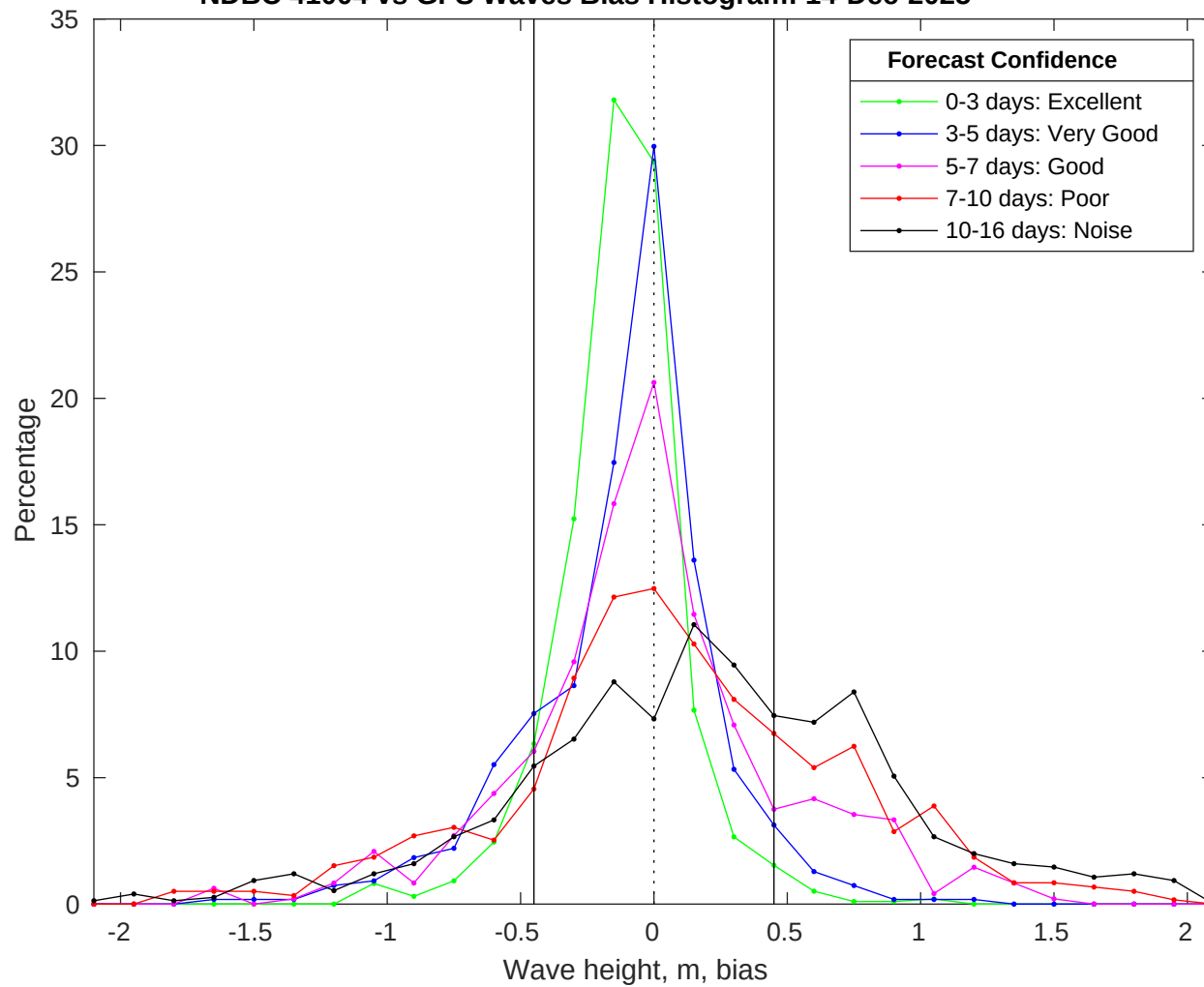
NDBC 41004 vs GFS Waves Bias Histogram: 14-Dec-2025
