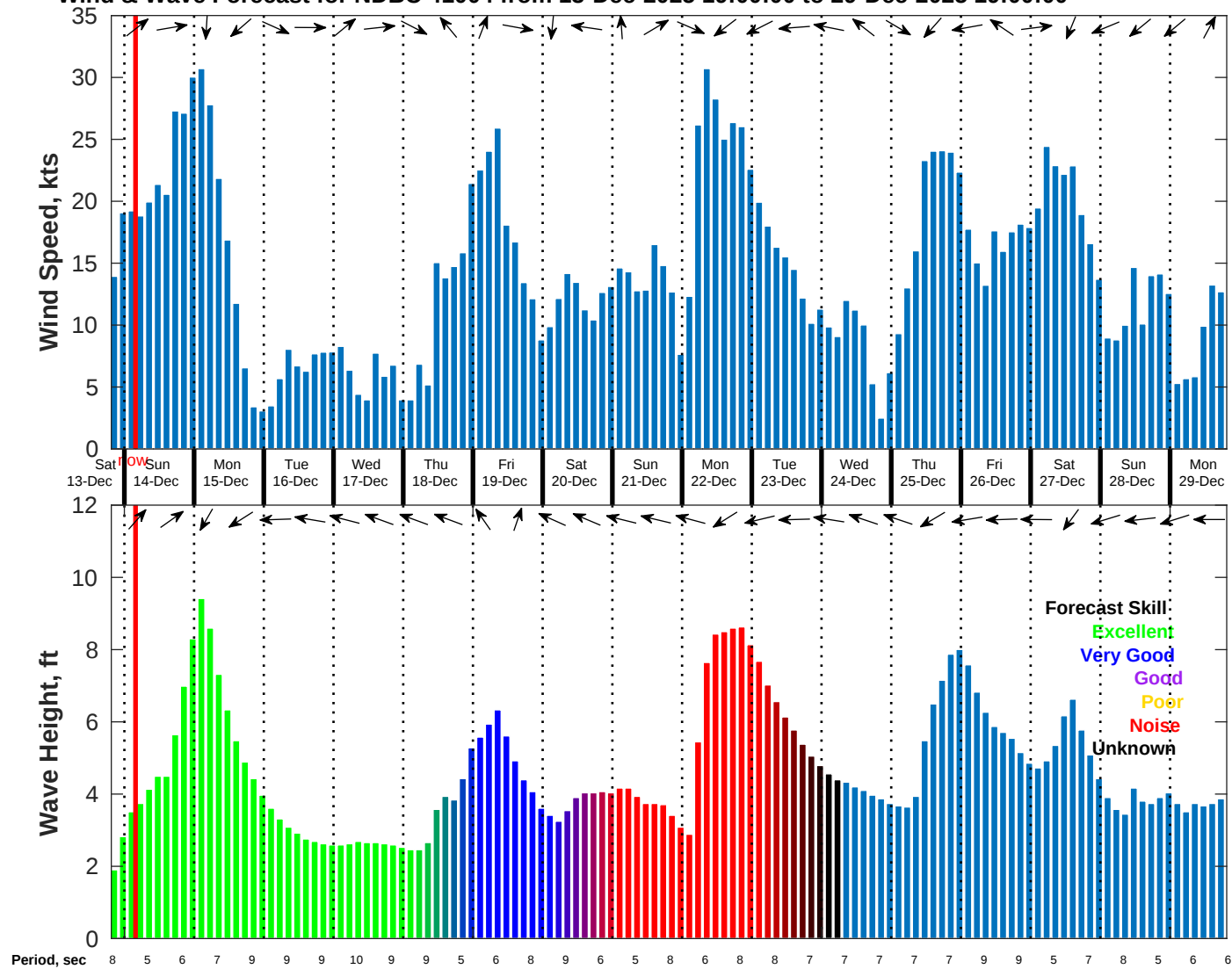
Wind & Wave Forecast for NDBC 41004 from 13-Dec-2025 19:00:00 to 29-Dec-2025 19:00:00
