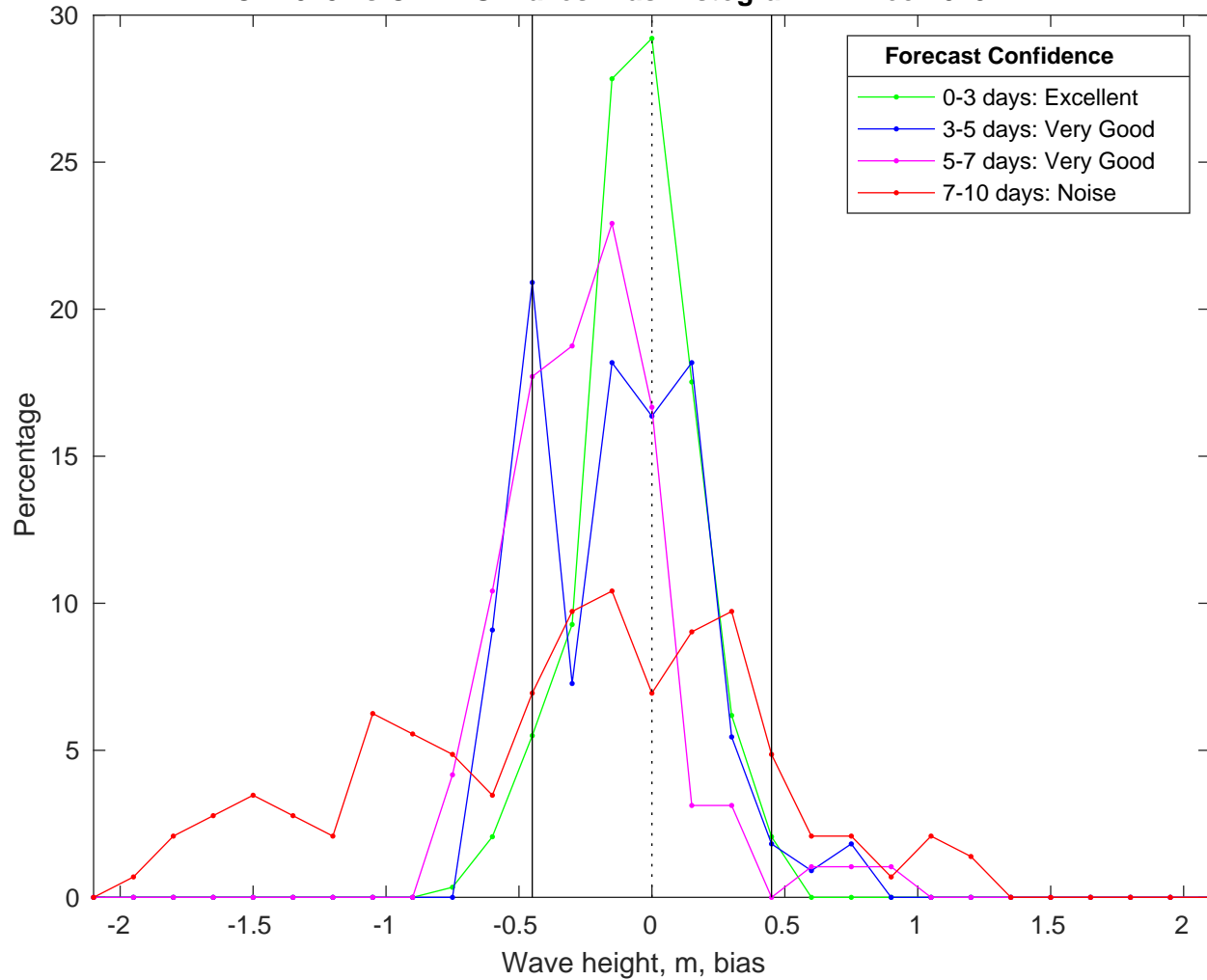
NDBC 41013 vs CMEMS Waves Bias Histogram: 14-Dec-2025
