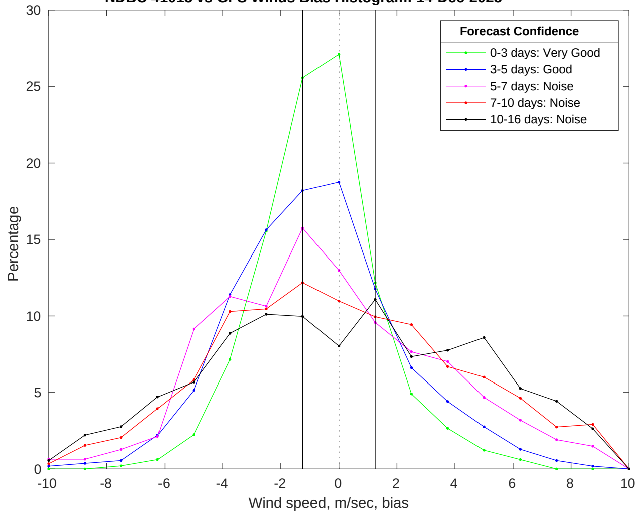
NDBC 41013 vs GFS Winds Bias Histogram: 14-Dec-2025
