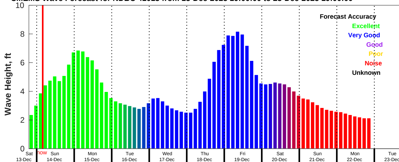
CMEMS Wave Forecast for NDBC 41013 from 13-Dec-2025 19:00:00 to 23-Dec-2025 19:00:00
