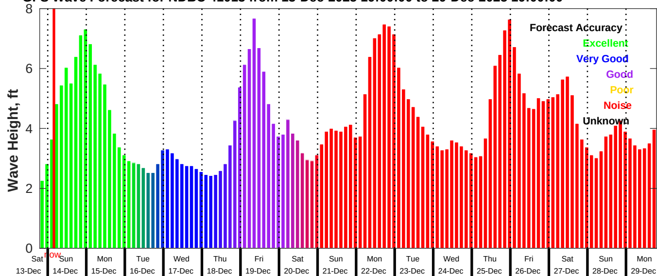
GFS Wave Forecast for NDBC 41013 from 13-Dec-2025 19:00:00 to 29-Dec-2025 19:00:00
