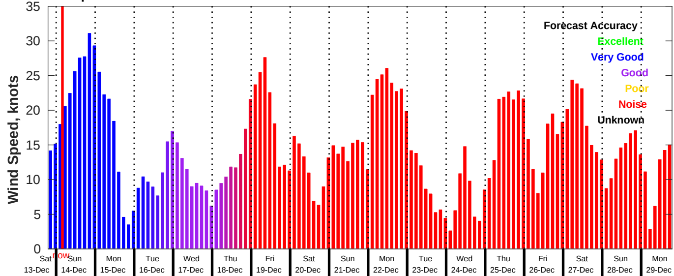
GFS Wind Speed Forecast for NDBC 41013 from 13-Dec-2025 19:00:00 to 29-Dec-2025 19:00:00
