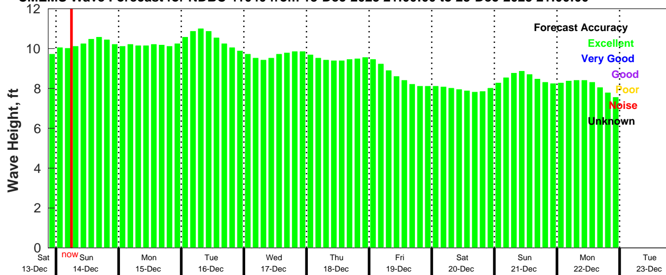
CMEMS Wave Forecast for NDBC 41040 from 13-Dec-2025 21:00:00 to 23-Dec-2025 21:00:00
