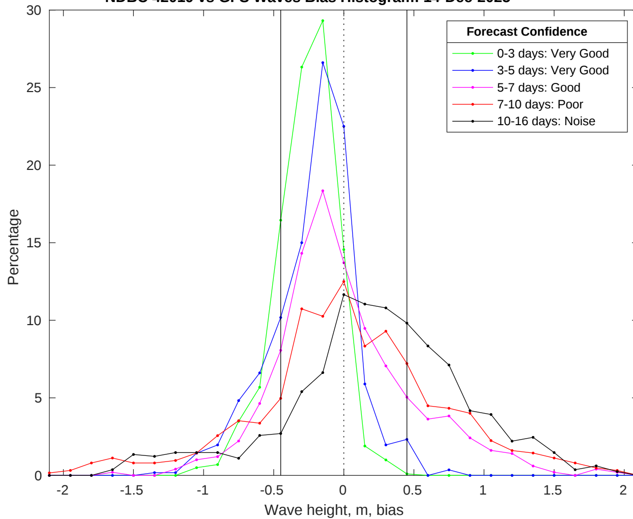
NDBC 42019 vs GFS Waves Bias Histogram: 14-Dec-2025
