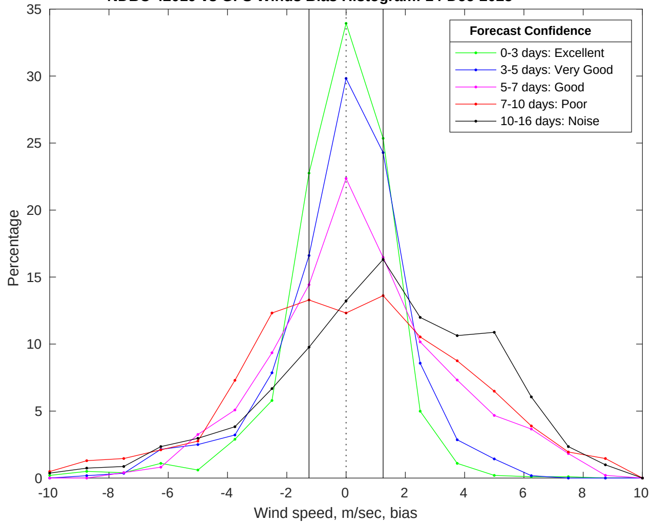
NDBC 42019 vs GFS Winds Bias Histogram: 14-Dec-2025
