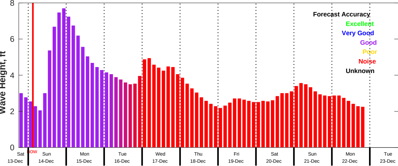
CMEMS Wave Forecast for NDBC 42020 from 13-Dec-2025 18:00:00 to 23-Dec-2025 18:00:00
