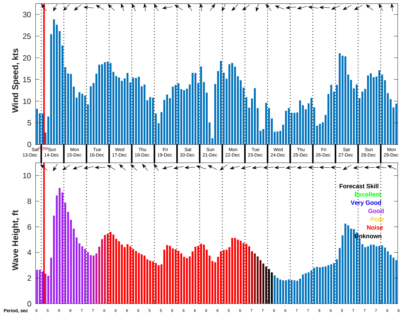
Wind & Wave Forecast for NDBC 42020 from 13-Dec-2025 18:00:00 to 29-Dec-2025 18:00:00
