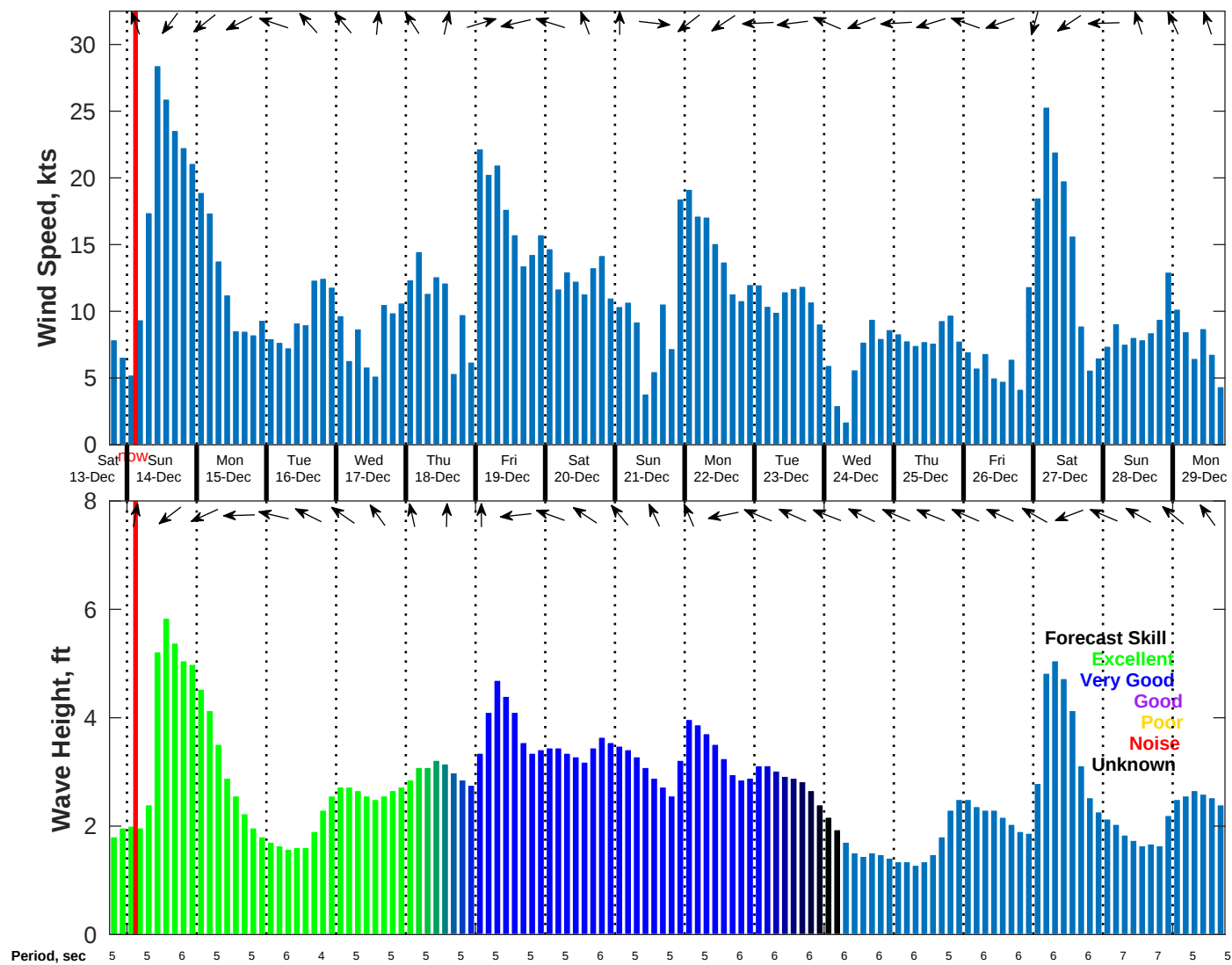
Wind & Wave Forecast for NDBC 42035 from 13-Dec-2025 18:00:00 to 29-Dec-2025 18:00:00
