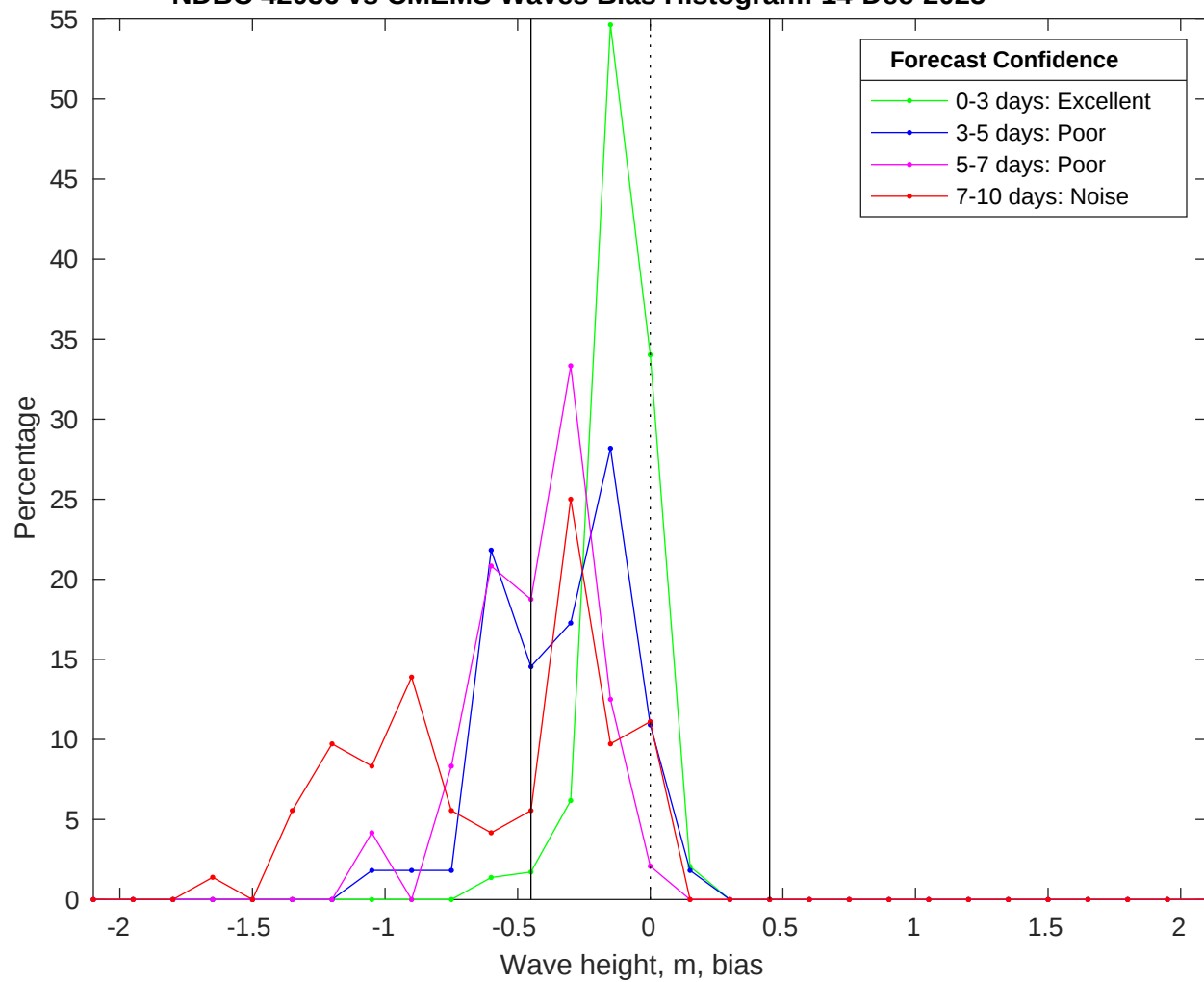
NDBC 42036 vs CMEMS Waves Bias Histogram: 14-Dec-2025
