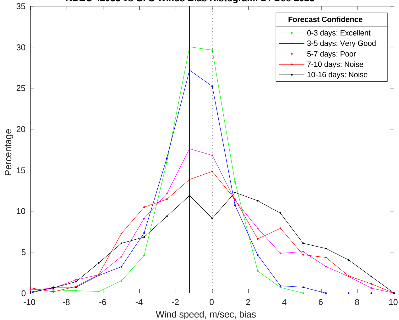
NDBC 42036 vs GFS Winds Bias Histogram: 14-Dec-2025
