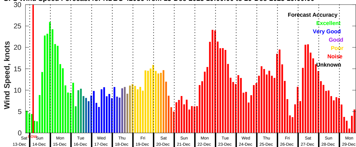
GFS Wind Speed Forecast for NDBC 42036 from 13-Dec-2025 19:00:00 to 29-Dec-2025 19:00:00
