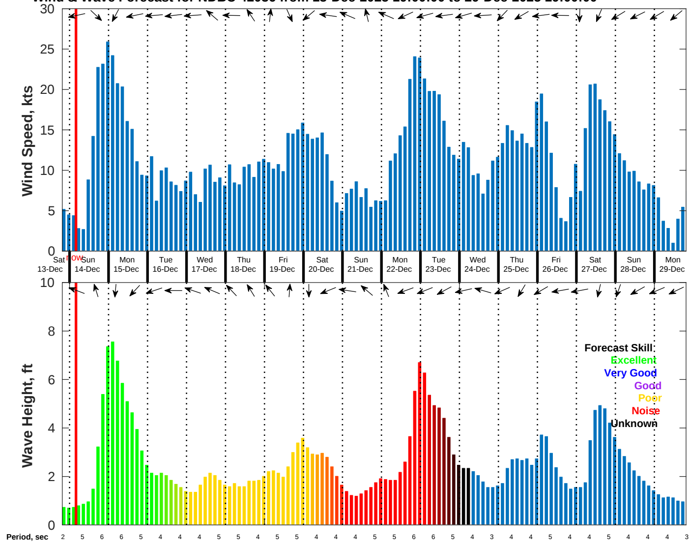
Wind & Wave Forecast for NDBC 42036 from 13-Dec-2025 19:00:00 to 29-Dec-2025 19:00:00
