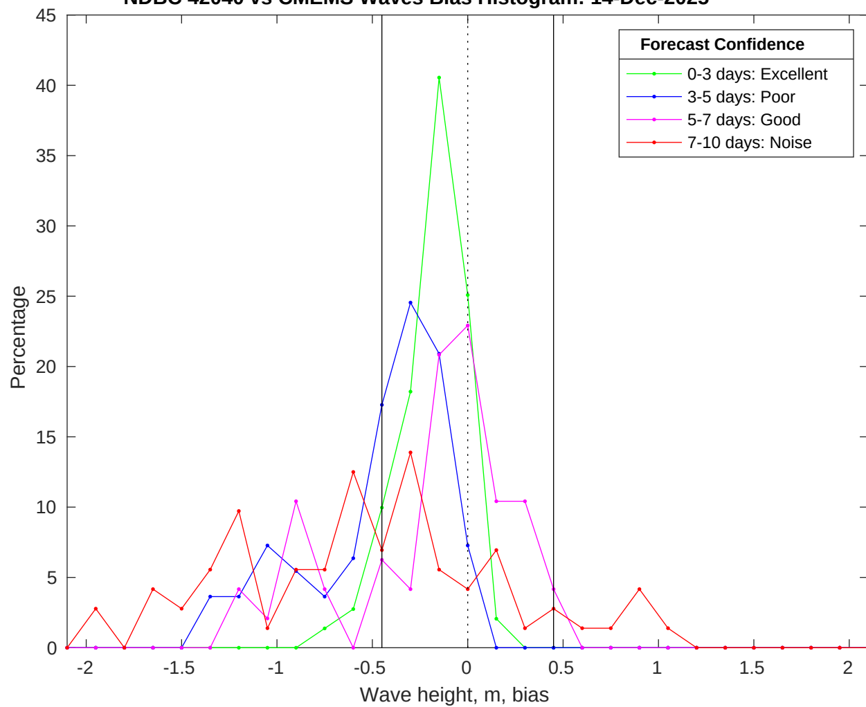
NDBC 42040 vs CMEMS Waves Bias Histogram: 14-Dec-2025
