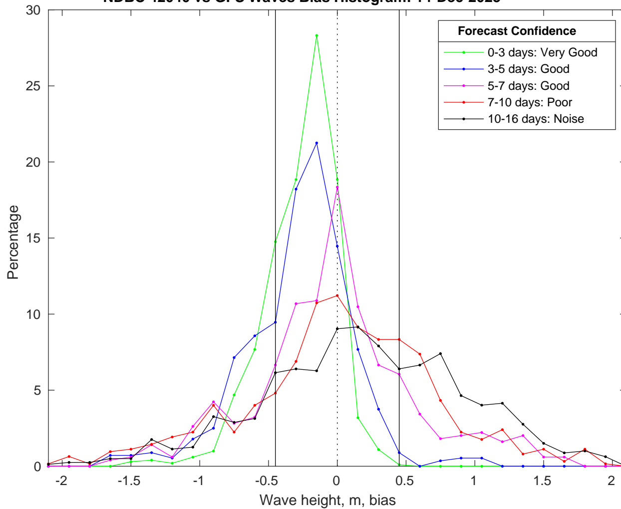
NDBC 42040 vs GFS Waves Bias Histogram: 14-Dec-2025
