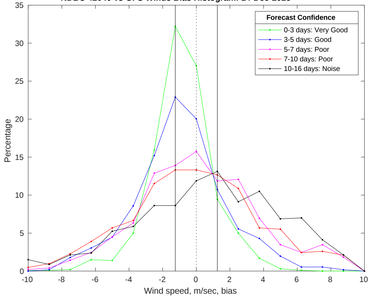
NDBC 42040 vs GFS Winds Bias Histogram: 14-Dec-2025
