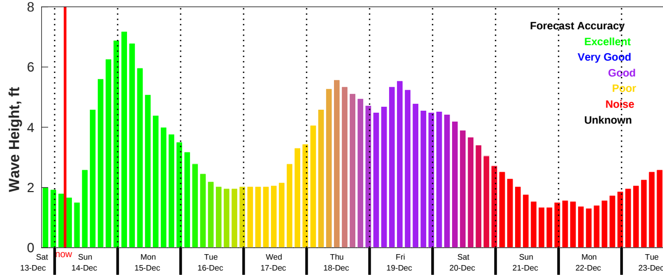
CMEMS Wave Forecast for NDBC 42040 from 13-Dec-2025 19:00:00 to 23-Dec-2025 19:00:00
