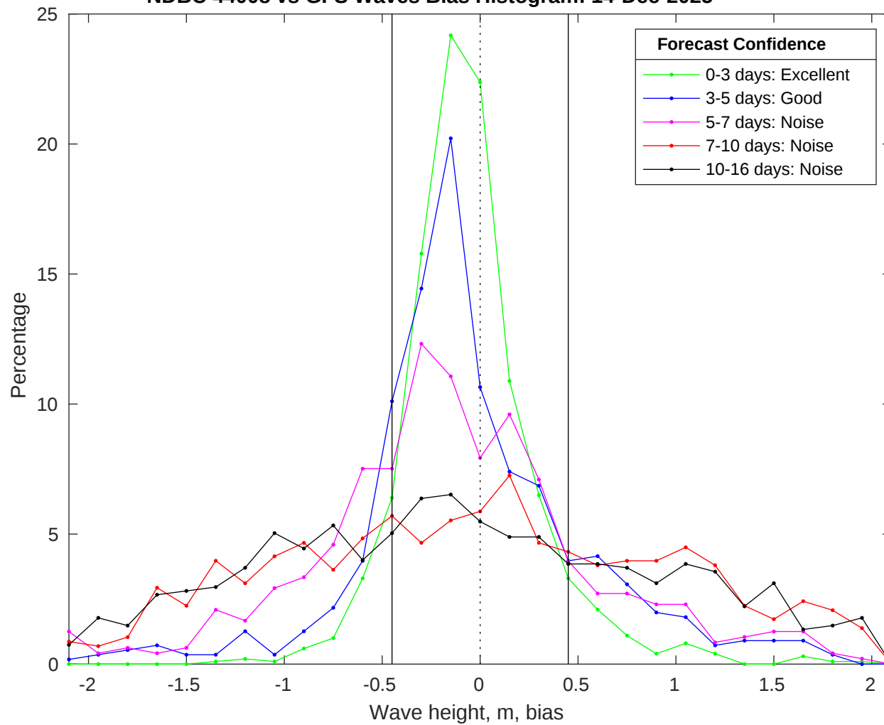
NDBC 44008 vs GFS Waves Bias Histogram: 14-Dec-2025
