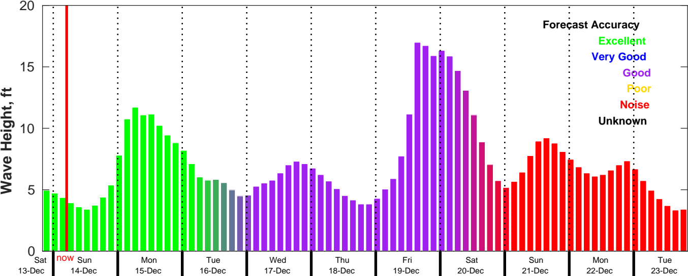
CMEMS Wave Forecast for NDBC 44008 from 13-Dec-2025 20:00:00 to 23-Dec-2025 20:00:00
