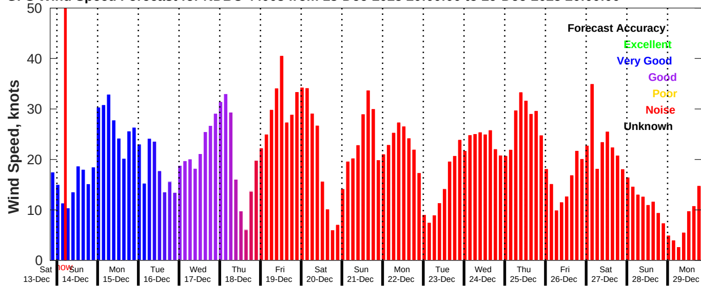
GFS Wind Speed Forecast for NDBC 44008 from 13-Dec-2025 20:00:00 to 29-Dec-2025 20:00:00
