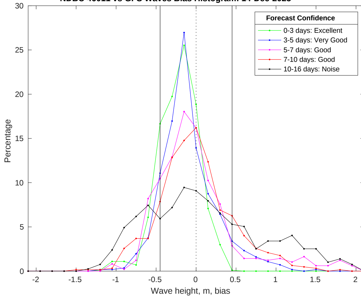
NDBC 46011 vs GFS Waves Bias Histogram: 14-Dec-2025
