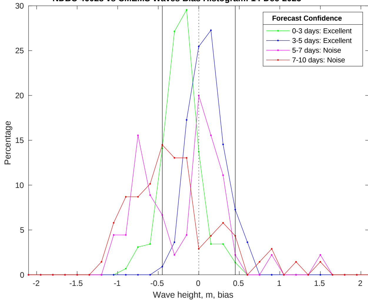
NDBC 46028 vs CMEMS Waves Bias Histogram: 14-Dec-2025
