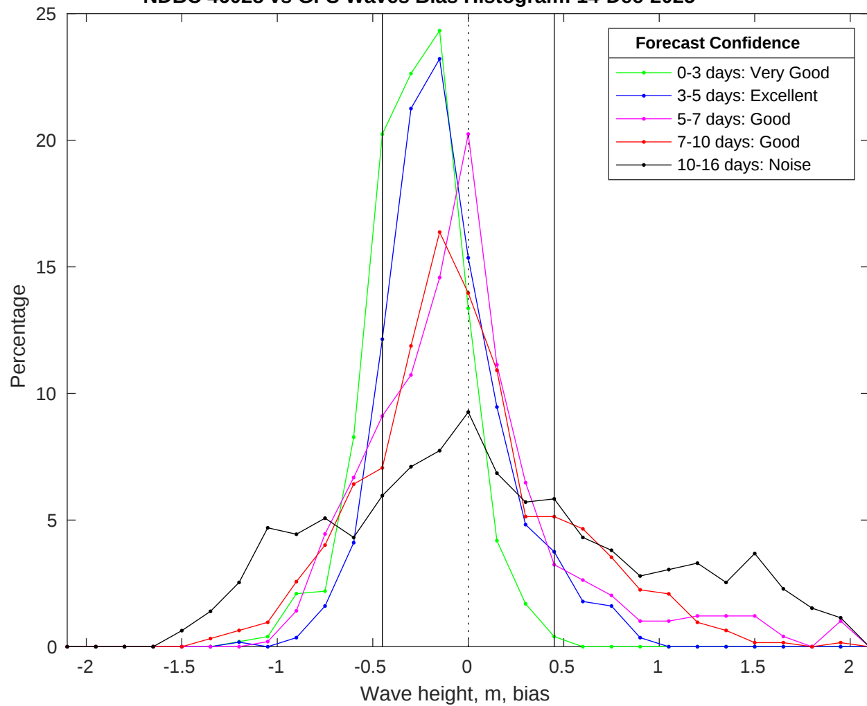
NDBC 46028 vs GFS Waves Bias Histogram: 14-Dec-2025
