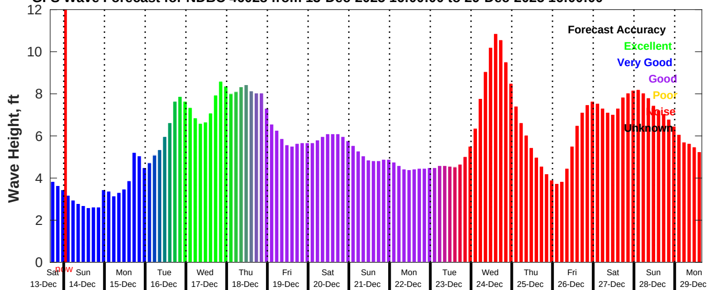
GFS Wave Forecast for NDBC 46028 from 13-Dec-2025 16:00:00 to 29-Dec-2025 16:00:00
