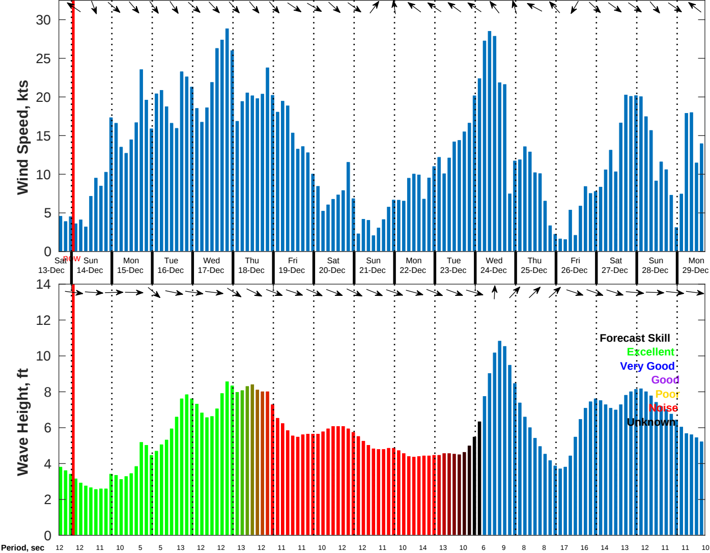
Wind & Wave Forecast for NDBC 46028 from 13-Dec-2025 16:00:00 to 29-Dec-2025 16:00:00
