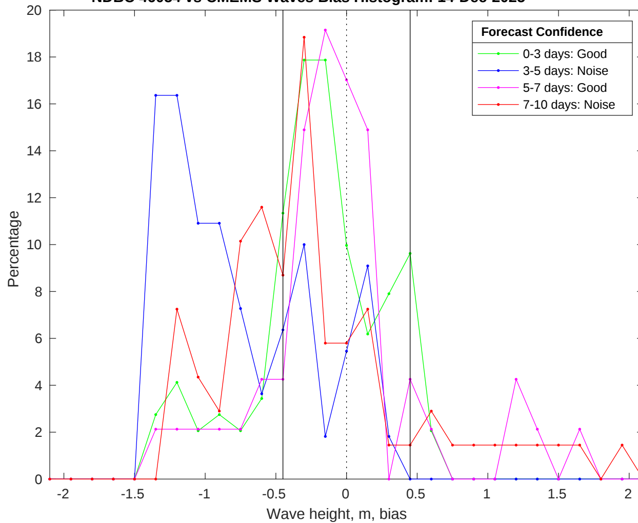
NDBC 46054 vs CMEMS Waves Bias Histogram: 14-Dec-2025
