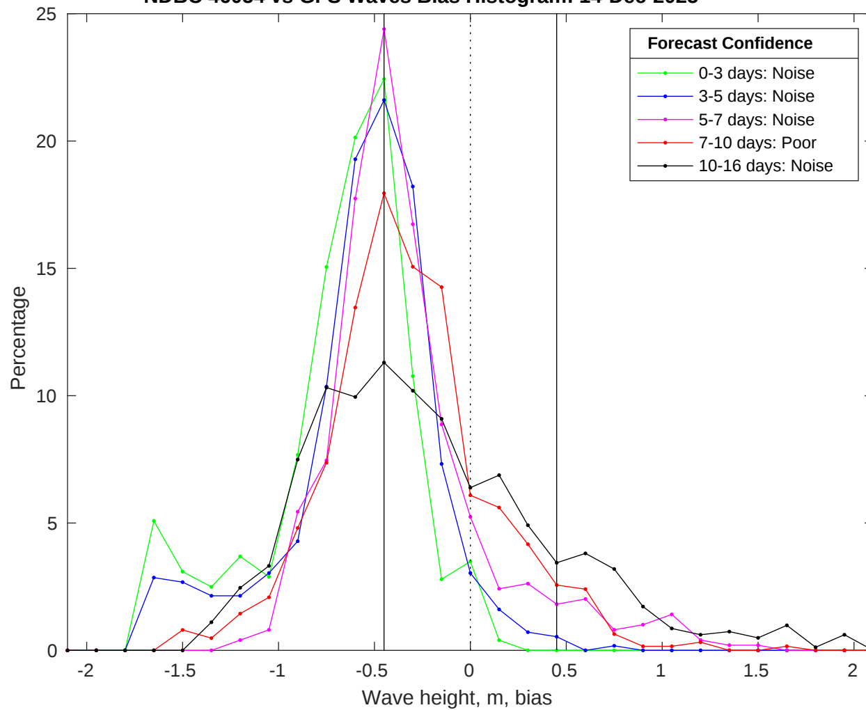
NDBC 46054 vs GFS Waves Bias Histogram: 14-Dec-2025
